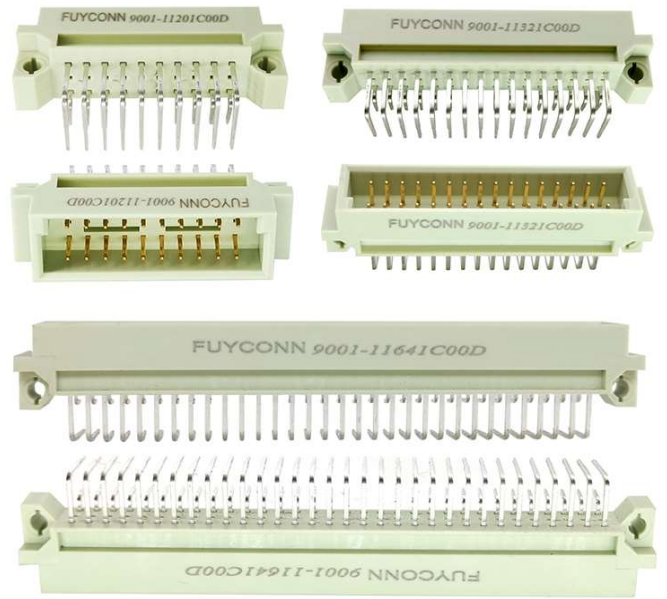
3 Rows Right Angle PCB Male Type
