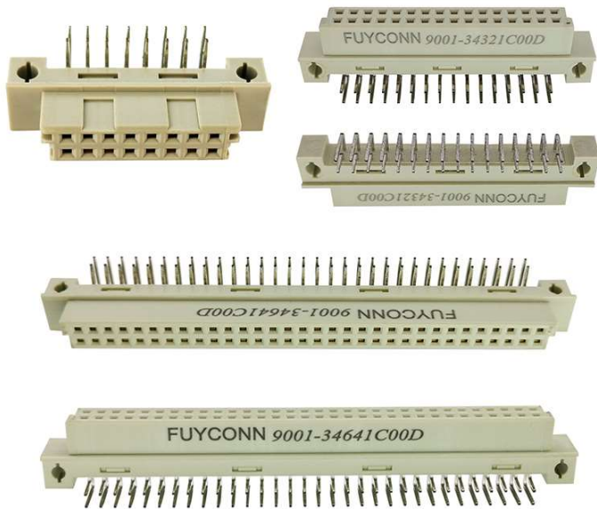
2 Rows Right Angle PCB Female Type
